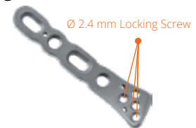
Locking Distal Ulna Plate
